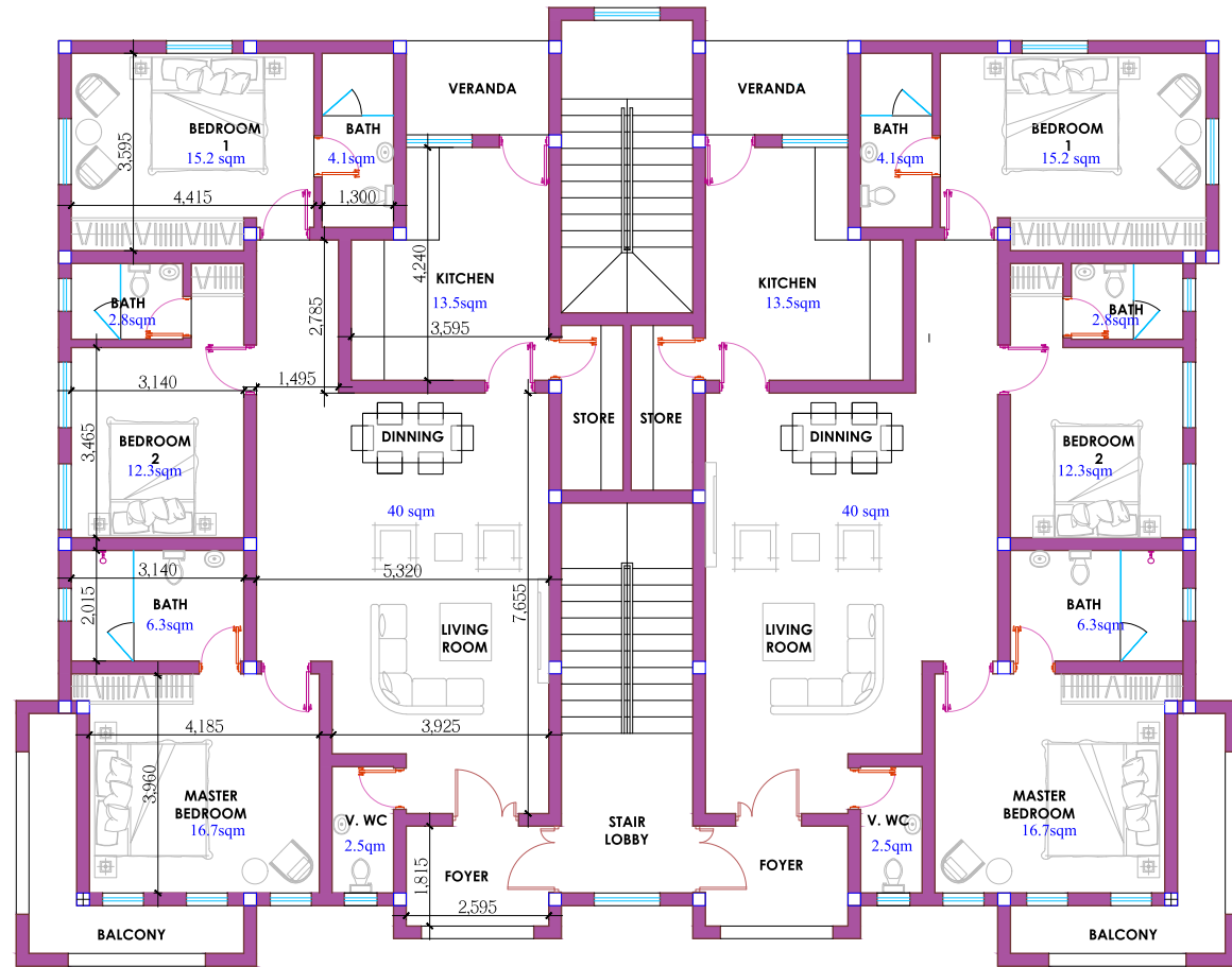
PROPOSED TYPICAL FLOOR PLAN
